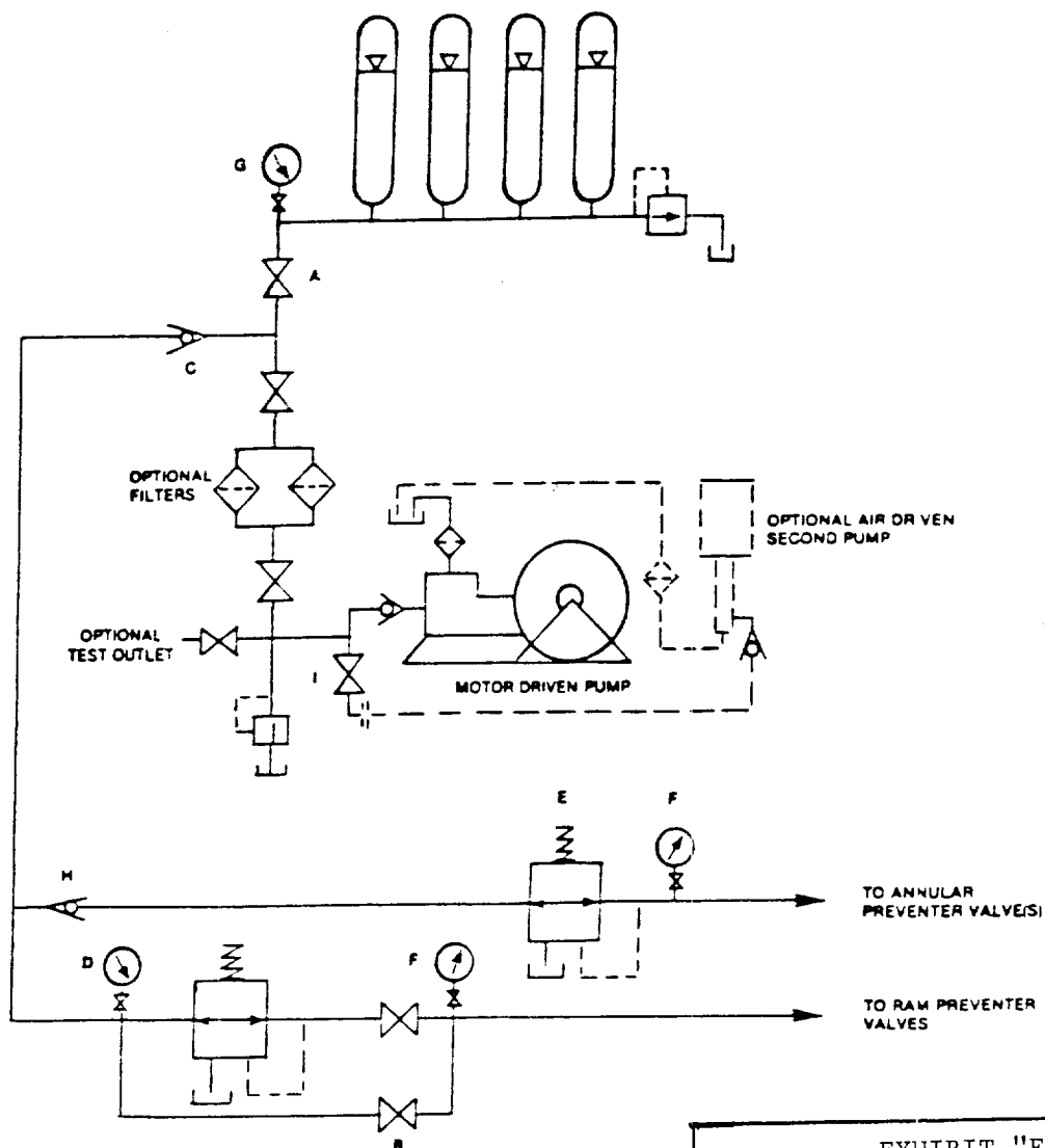
EXHIBIT "E-1" CHOKES MANIFOLD & CLOSING UNIT
