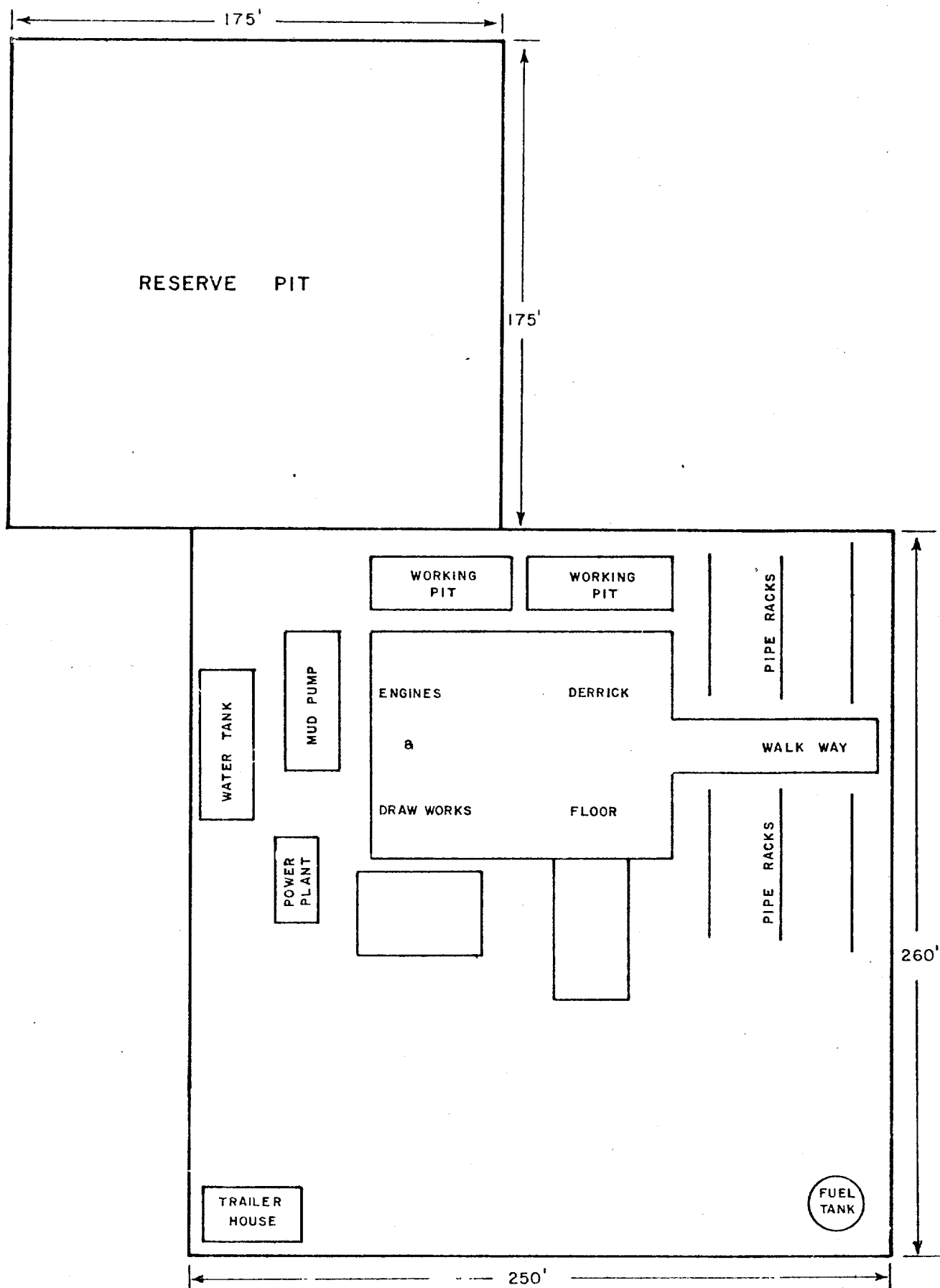
APPROXIMATE LOCATION SIZE 8 APPROXIMATE RIG LAYOUT
