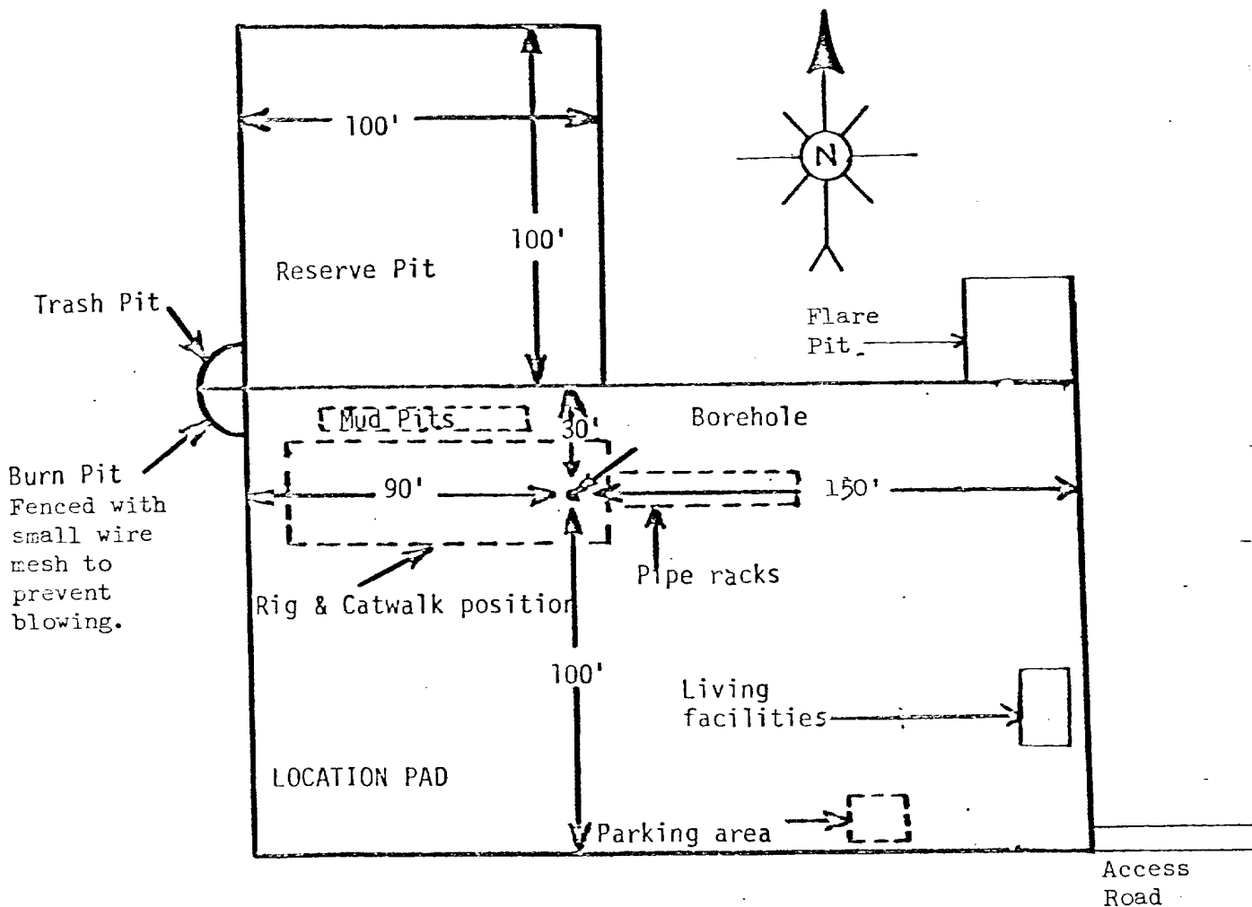
EXHIBIT "A" Rig layout for Leonard Bros. well # 19
