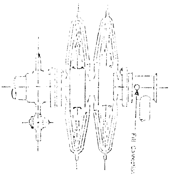
Shafter Type E Series 900 Hydraulic BOP
