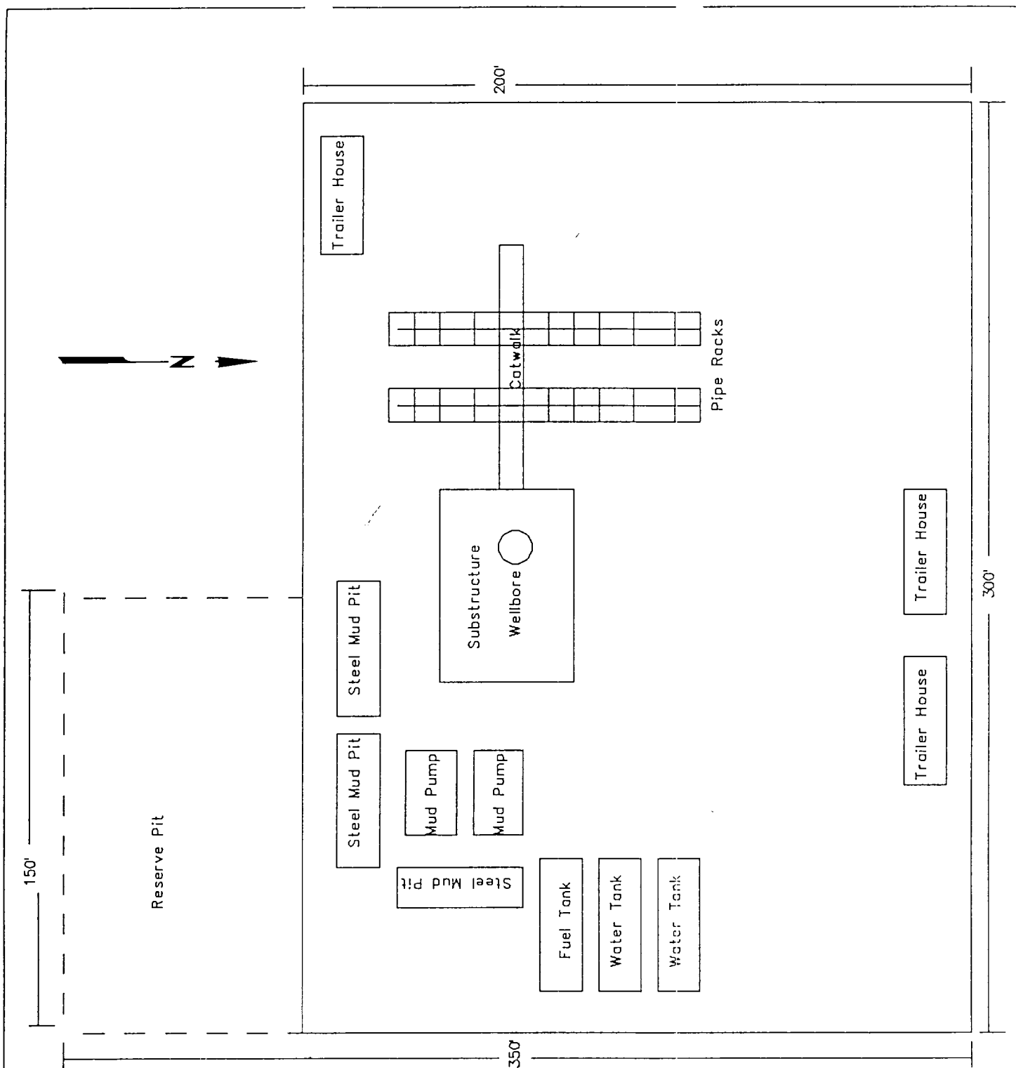
EXHIBIT G WELL SITE LAYOUT SANTA FE ENERGY RESOURCES, INC. Mesa Verde "6" FEDERAL NO. 10 330' FNL & 330' FWL SECTION 6, T-24-S, R-32-E LEA COUNTY, NEW MEXICO
