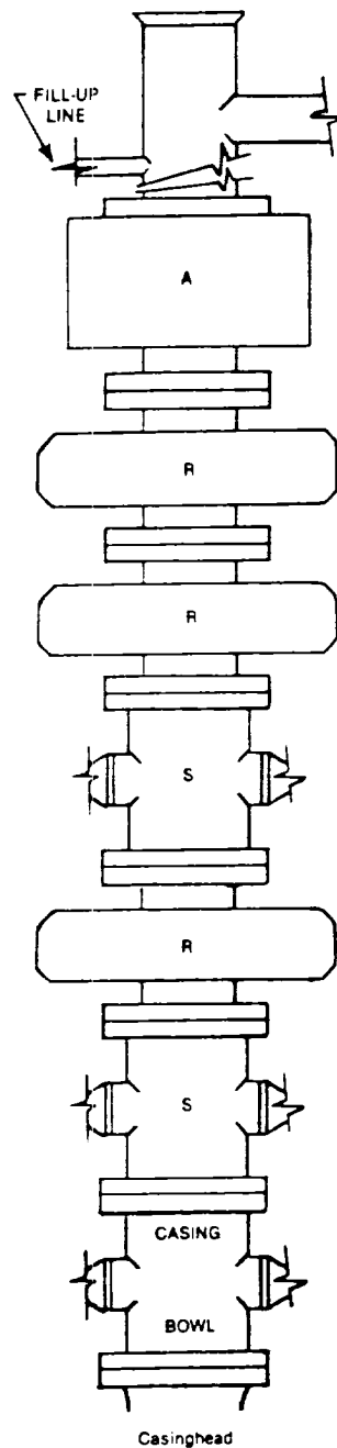
FIGURE K1-3. Recommended IADC Class 10 BOP stack arrangement SRSRRA, 10,000 psi WP. Lower drilling spool is optional with outlets on lower ram. Annular preventers 10,000 psi.
