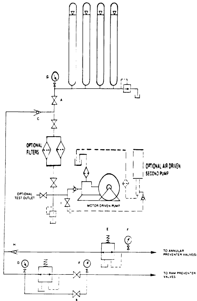
FIGURE K6-1. The schematic sketch of an accumulator system shows required and optional components.
