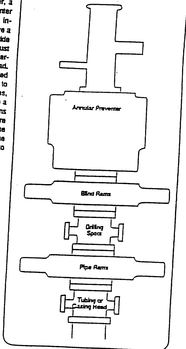
Figure 11J.4 Class III Blowout Preventer Stack
