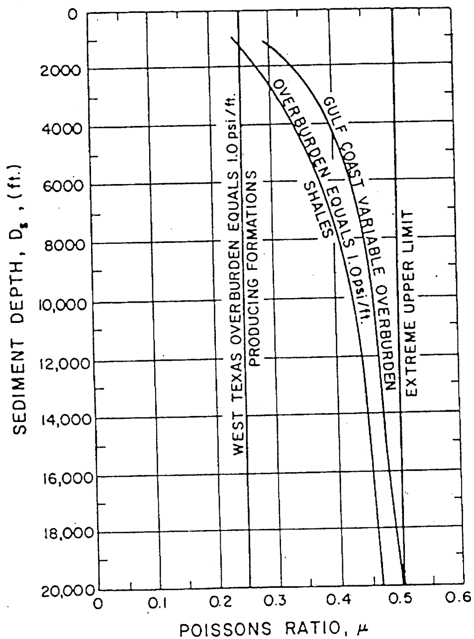
Fig. 6.50—Eaton correlation for Poisson's ratio. 1
