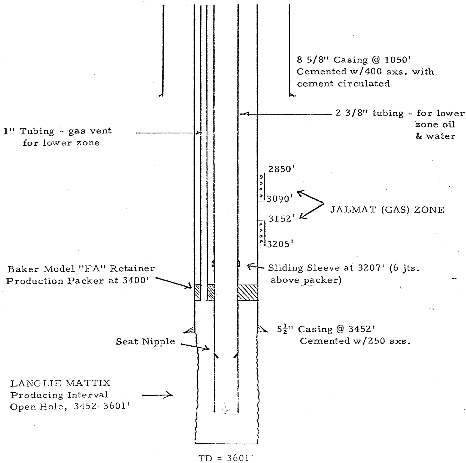
WELLBORE DIAGRAM
