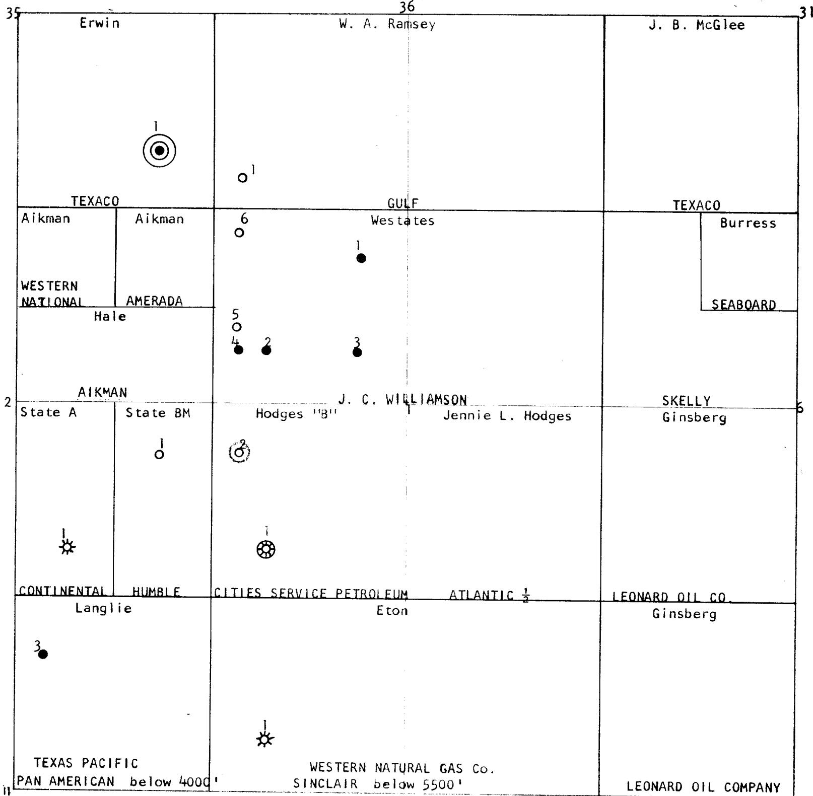
12 Plat Showing the Proposed Dual Completion, Hodges B #2 and off- set operators
