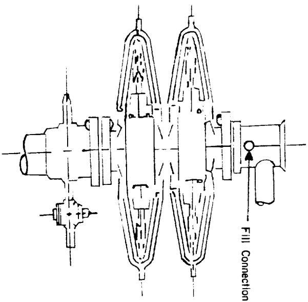
Shafter Type E Series 900 Hydraulic B.O.P
