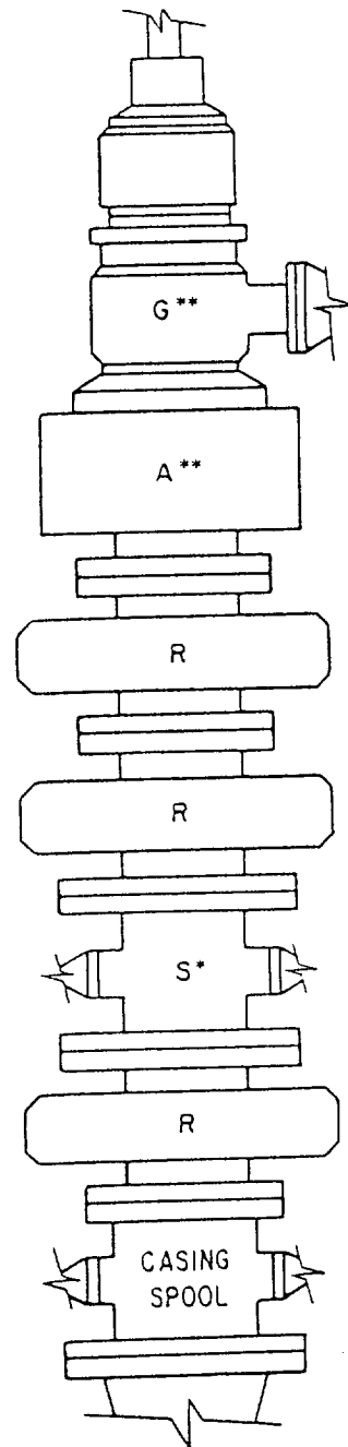
FIG. 2.C.9 ARRANGEMENT RS*RA**G** Double Ram Type Preventers, R d , Optional
