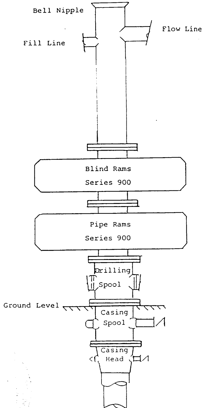
BLOWOUT PREVENTER STACK
